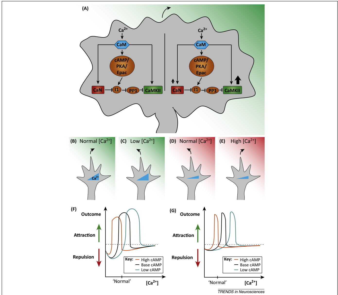
Figure 2. A mathematical model for how calmodulin-dependent protein kinase II (CaMKII) and calcineurin (CaN) activity modulation determines growth cone attraction versus repulsion to a gradient [42]. (A) The growth cone is imagined to be split into two compartments (up-gradient to the right, and down-gradient to the left). On each side a Ca^{2+} -dependent switch [47] processes Ca^{2+} elevations. Calcium binds to CaM to form a calcium/CaM complex which activates CaN, protein kinase A (PKA), and CaMKII. At low concentrations of calcium ( [Ca^{2+}] ), CaMKII has low affinity for the calcium/CaM complex, and CaN activity therefore predominates. As the calcium concentration rises above a threshold, the affinity of the calcium/CaM complex for CaMKII increases dramatically, resulting in a higher activity of CaMKII compared to CaN. The model compares the ratios of CaMKII:CaN between the two sides of the growth cone, and hypothesizes that turning occurs to the side with the higher ratio. (B–E) Summary of experimental findings regarding how the steepness of the intracellular Ca^{2+} gradient interacts with background concentrations of Ca^{2+} to determine the direction of turning. (F) Predictions of the model for a normally attractive gradient. At normal PKA levels (black curve) and normal background Ca^{2+} concentrations the ratio of CaMKII:CaN is higher on the up-gradient side (assumed to have 30% higher Ca^{2+} ) compared to the down-gradient side of the growth cone, and thus the response is attraction. However, in low background Ca^{2+} , CaMKII is very low on both sides, whereas CaN is still increasing with Ca^{2+} concentration. This causes the ratio of CaMKII:CaN to be higher on the down-gradient (lower Ca^{2+} ) side, leading to repulsion. In high background Ca^{2+} the activity of CaMKII is saturated on both sides, and the steady increase of CaN with Ca^{2+} concentration means that again the CaMKII:CaN ratio is now higher on the down-gradient side, leading to repulsion. The effect of changing PKA activity is primarily to shift the curve along the Ca^{2+} concentration axis. When this shift is large enough it causes both high and low levels of PKA to lead to repulsion. (G) Predictions of the model for a normally repulsive gradient. In this case the up-gradient side is assumed to have 10% higher Ca^{2+} . Similar reasoning applies as for the normally attractive gradient discussed above, but the response at normal background Ca^{2+} concentration is now repulsion because the 10% increase is not sufficient to cause a large increase in CaMKII activity between the two sides; [42] for more details. Abbreviations: Epac, exchange protein directly activated by cAMP; I1, inhibitor 1; PKA, protein kinase A; PP1, protein phosphatase 1.
