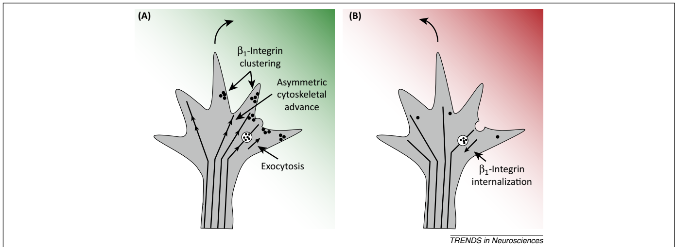
Figure 3. \beta_1 -Integrins and membrane dynamics in response to calcium signaling during growth cone guidance. (A) Attractive chemotropic cues induce asymmetric exocytosis in the growth cone mediated by vesicle-associated membrane protein 2 (VAMP2) or syntaxin and neurotoxin-insensitive VAMP (TI-VAMP), as well as by \beta_1 -integrin clustering on the cell plasma membrane on the up-side of the gradient. Increased actin polymerization and branching, as well as increased tubulin polymerization, lead to an asymmetric increase in filopodial and lamellipodial activity on the up-side of the gradient. \text{Ca}^{2+} functions as a second messenger that directly activates these components. Increased adhesion of the growth cone to the substrate via \beta_1 -integrin, and addition of new plasma membrane to the up-side of the gradient, leads to turning and increased axon outgrowth in response to gradients of attractive guidance cues such as brain-derived neurotrophic factor (BDNF; green). (B) By contrast, gradients of repulsive chemotropic cues such as myelin-associated glycoprotein (MAG; red) lead to internalization of \beta_1 -integrin via clathrin-mediated endocytosis, as well as the asymmetric endocytosis of cell plasma membrane on the up-side of repulsive guidance cue gradients. Loss of \beta_1 -integrin adhesions and removal of the cell membrane leads to turning of the growth cone away from the gradient.
