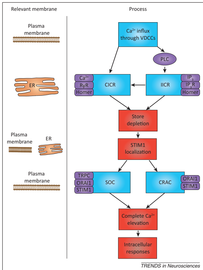
Figure 1. Pathways of calcium entry into growth cones and release from intracellular stores. Calcium entry occurs through VDCCs (in particular L-type calcium channels) in the cell plasma membrane to activate CICR directly, and indirectly initiate IICR. CICR and IICR are both Homer1-mediated and release \text{Ca}^{2+} from the ER. CICR is induced by the binding of incoming \text{Ca}^{2+} to RyRs on the ER membrane. In the \text{IP}_3 pathway, PLC is activated to hydrolyze \text{PIP}_2 into \text{IP}_3 and diacylglycerol. \text{IP}_3 binds to receptors on the surface of the ER, initiating IICR. In response to calcium store depletion, STIM1 becomes localized to the ER and plasma membrane junctions, and leads to SOCE through SOC channels which utilize TRPC and ORAI1, and CRAC channels which depend mainly on ORAI1. SOCE facilitates large influxes of \text{Ca}^{2+} from extracellular sources. The resulting asymmetric intracellular calcium elevation leads to asymmetric intracellular responses creating attraction or repulsion. Colors indicate the function of a component: purple for important molecules, blue for calcium-releasing processes and red for other processes. The left column indicates major membranes involved in each step. Abbreviations: ER, endoplasmic reticulum; CICR, calcium-induced calcium release; CRAC, calcium release-activated channel; IICR, \text{IP}_3 -induced calcium release; \text{IP}_3 , inositol trisphosphate; \text{IP}_3\text{R} , \text{IP}_3 receptor; ORAI1, calcium release-activated calcium channel protein 1; PLC, phospholipase C; \text{PIP}_2 , 4,5-bisphosphate; RyR, ryanodine receptor; SOC, store-operated calcium; SOCE, store-operated calcium entry; STIM1, stromal interaction molecule 1; TRPC, transient receptor potential cation channel; VDCC, voltage-dependent calcium channel.
